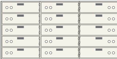
SDX-15 15 openings ea. 3" x 10"
